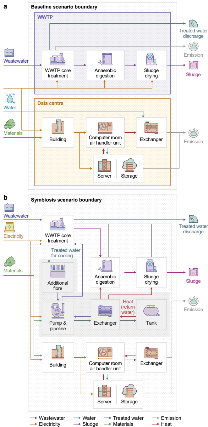
Fig. 1. Life-cycle assessment boundary for the data centre and wastewater treatment plant (WWTP) in the baseline and symbiosis scenario. a. Baseline scenario; b. Symbiosis scenario. The baseline scenario shows the data centre and WWTP operating independently, with the data centre relying on a freshwater supply and the WWTP discharging treated effluent directly. The symbiosis scenario illustrates the integrated operations: (1) treated water from the WWTP undergoes tertiary treatment (additional filtration) to replace freshwater for the data centre cooling; (2) waste heat from the data centre is recovered via heat exchangers and returned to the WWTP to support anaerobic digestion and sludge drying. The grey shaded area represents the foreground infrastructure added to enable the symbiosis (e.g., pumps, pipelines, and exchangers). Colored arrows indicate the direction of water, electricity, materials, and heat flows between unit processes. This schematic illustrates a representative one-to-one pairing to highlight the coupling mechanism; actual matches in the study may involve one-to-many or many-to-one configurations. The assumed operational lifespan is 20 years, with a functional unit of 1 kWh of IT load.
