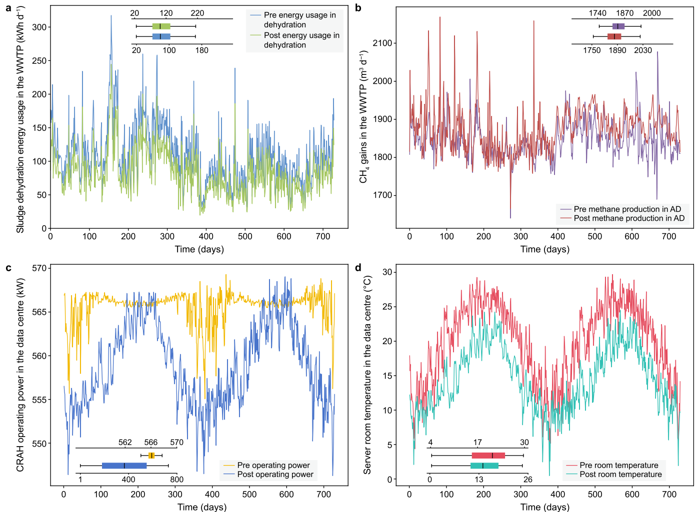
Fig. 4. Long-term performance of the co-construction of the data centre and WWTP process configuration. This configuration comprises four interlinked technological components (CRAH, AOA unit, anaerobic digestion and sludge dehydration) to enable smooth operation and maintenance. The data centre's CRAH generates a significant volume of heated water, which is then directed to the WWTP's anaerobic digestion unit and the sludge dehydration heat exchanger. a , Time-series variation in sludge-drying energy consumption, showing the reduction achieved under the co-construction scenario relative to the baseline scenario. b , Time-series variation in methane production from the WWTP, showing the enhancement associated with thermally supported anaerobic digestion. c , Time-series variation in CRAH power demand, showing the reduced cooling energy demand under the chiller-less co-construction configuration. d , Time-series variation in server-room temperature, showing the thermal response and stability of the data-centre operation under the co-construction scenario. Insets in a–d summarize the mean and variance of the corresponding colored traces in each panel. The inset y axis represents the same variable as that in the corresponding main panel, and the unit is identical to that of the corresponding main-panel y axis.
