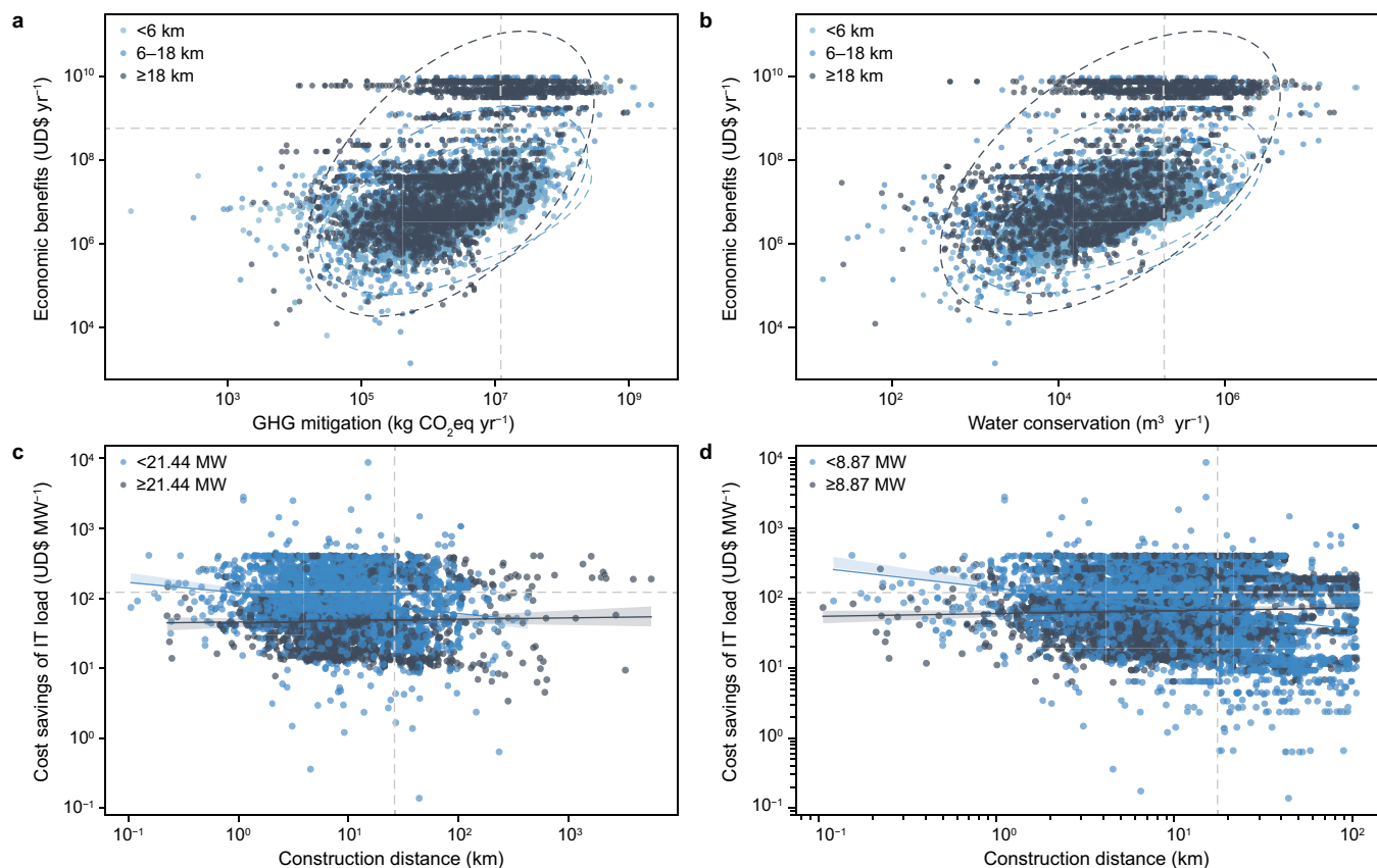
Fig. 3. The impact of co-construction on the environment and economy. a–b. Greenhouse gas (GHG) mitigation ( a ) and freshwater conservation ( b ) versus cost reductions of each energy recycling linkage. c. Data centre-aggregated cumulative pipeline length versus cost reductions per megawatt (MW) IT load. d. Pipeline-level length versus cost reductions per MW IT load. The points representing GHG, freshwater conservation, and cost linkages are categorised by the distance between data centres and WWTPs. Horizontal and vertical grey dashed lines indicate the mean values of the variables on the y and x axes, respectively, in each panel. In a and b , dashed ellipses indicate the 95% covariance ellipses of linkage-level observations for the three pipeline-distance groups (<6 km, 6–18 km, and ≥18 km), calculated in log-transformed space and shown on log-scaled axes. They summarize the group-specific centroid, spread, and orientation of the bivariate distribution. In c , the solid lines show how the relationship between cumulative pipeline length and cost savings per MW of IT load varies across different capacity classes at the data centre level; in d , the solid lines show the corresponding relationship at the individual pipeline level. Shaded bands indicate the 95% confidence intervals of the fitted relationships. The benefit per m 3 of wastewater recovered represents the net cost reduction after accounting for sludge dewatering and anaerobic digestion; the cost reduction per megawatt of computing power represents the net cost reduction after accounting for changes in industrial water use, water pipeline construction and operation, and data centre advanced wastewater treatment costs.
